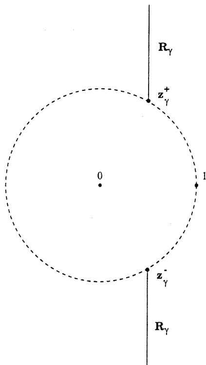
Figure 1. The set \mathbb{C} \setminus \mathbb{R}_\gamma .
