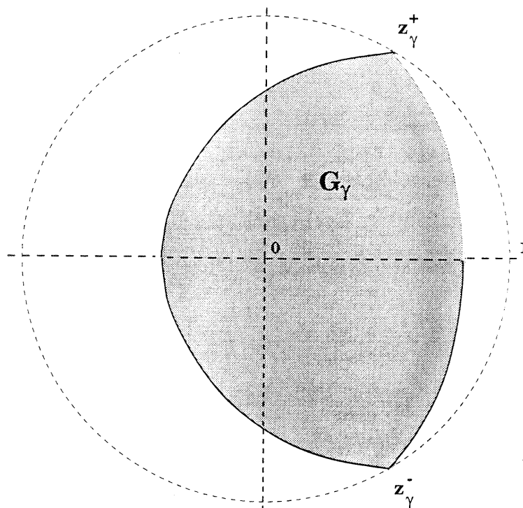
Figure 2. The set G_\gamma .
