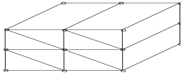
FIG. 8.1. A three-dimensional mixed finite element with discontinuous pressures.
