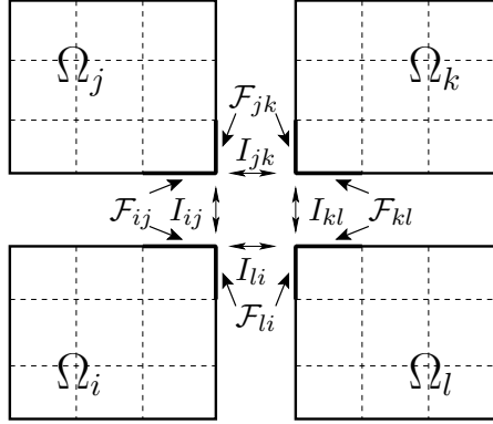
FIG. 3.1. Illustration on a subdomain edge interface degree of freedom.
