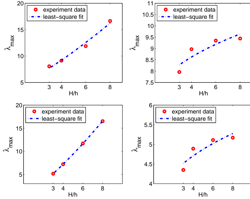
FIG. 8.2. Least squares fits of \lambda_{max} in Table 8.3 (top row) and in Table 8.4 (bottom row) with respect to H/h by C_1\alpha + C_2(H/h)(1 + \log(H/h)) for the lumped preconditioner (left) and by C_1\alpha + C_2(1 + \log(H/h))^2 for the Dirichlet preconditioner (right).
