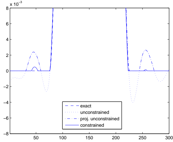
Fig. 4. Example 1: Magnification of part of Figure 3.
