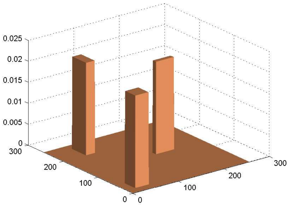
Fig. 9. Example 3: Blur- and noise-free surface.
