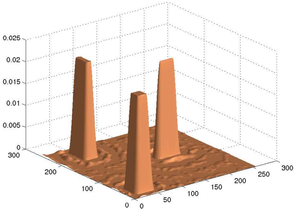
Fig. 11. Example 3: Restored surface represented by \tilde{\mathbf{x}}^+ , \gamma = 1.0 \cdot 10^{-2}
