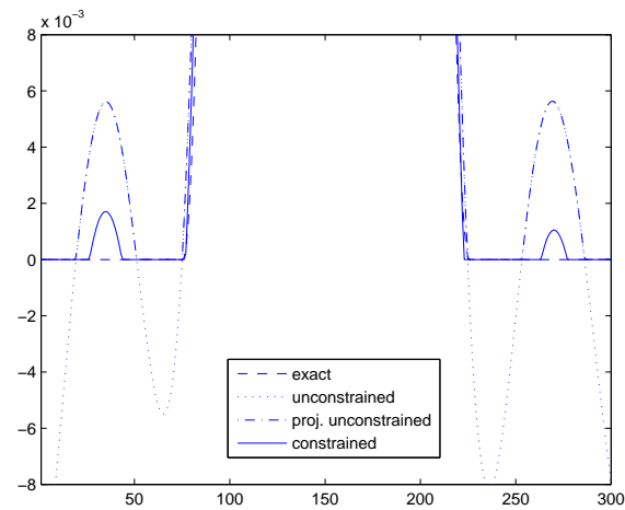
Fig. 1. Example 1: Exact and computed approximate solutions for \gamma = 0.1 .
