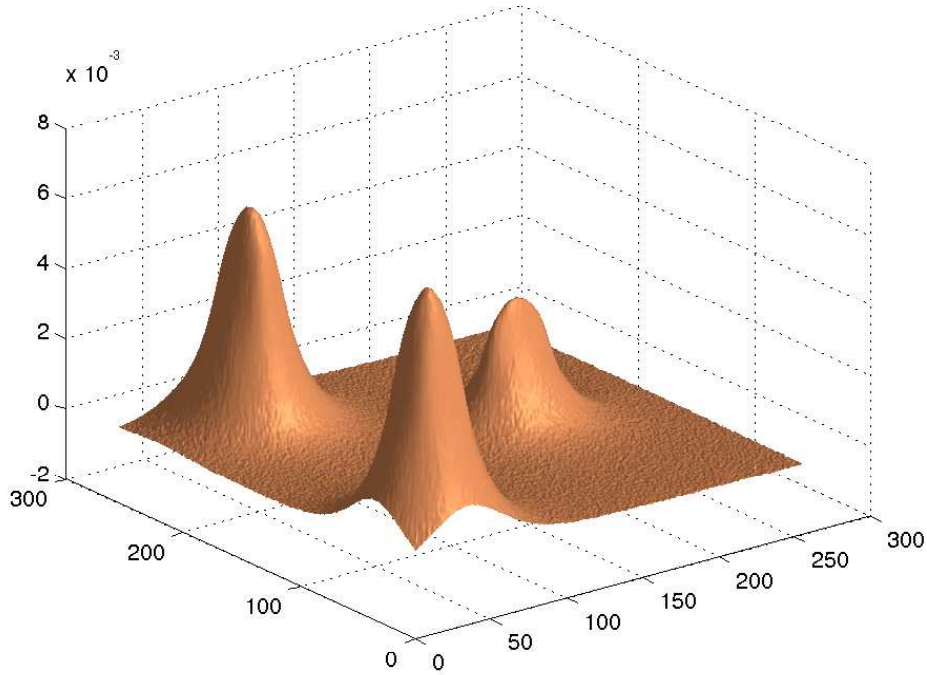
Fig. 10. Example 3: Blurred and noisy surface, \gamma = 1.0 \cdot 10^{-2} .
