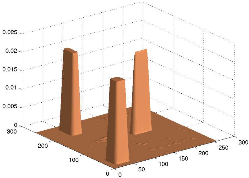
Fig. 12. Example 3: Restored surface represented by \hat{\mathbf{x}} , \gamma = 1.0 \cdot 10^{-2} .
