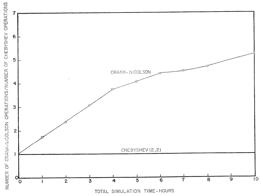
FIG. 3. Comparison of Number of Operations—Crank-Nicolson Method vs. Chebyshev Method ( L_\infty Norm = 17.4 psi).
