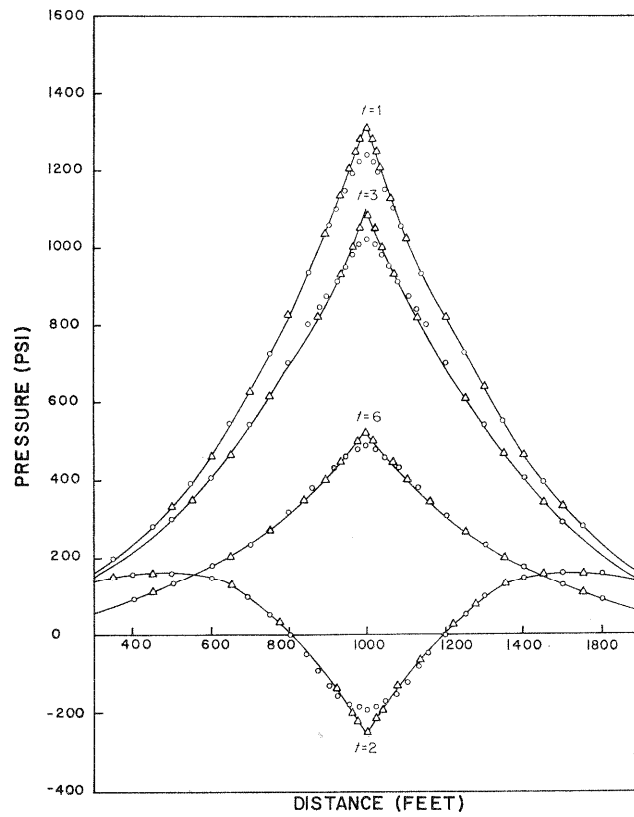
FIG. 5. Numerical Solutions to Eq. (16) Using Table IV Data ( \Delta — (2,2) Chebyshev Method; \circ — Crank-Nicolson Method ( \Delta t = 0.25 ); — Exact Solution).
