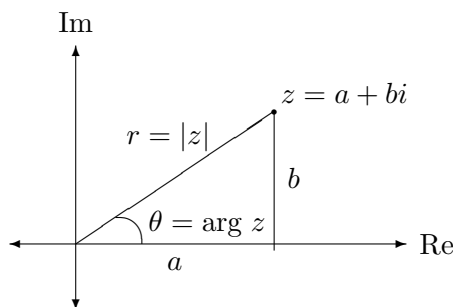
Figure 1.4: Polar Form of Complex Numbers
