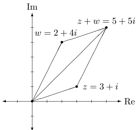
Figure 1.2: Addition of Complex Numbers
