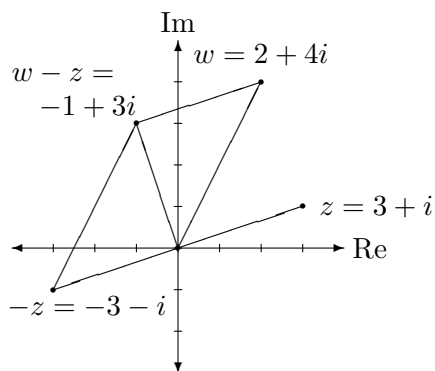
Figure 1.3: Subtraction of Complex Numbers
