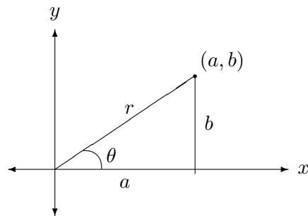
Figure B.1: Polar Coordinates of a Point
