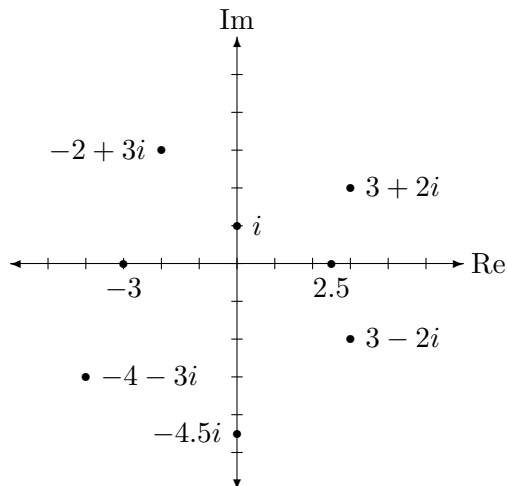
Figure 1.1: The Complex Plane
