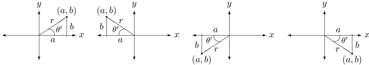
Figure B.2: Reference Angles
