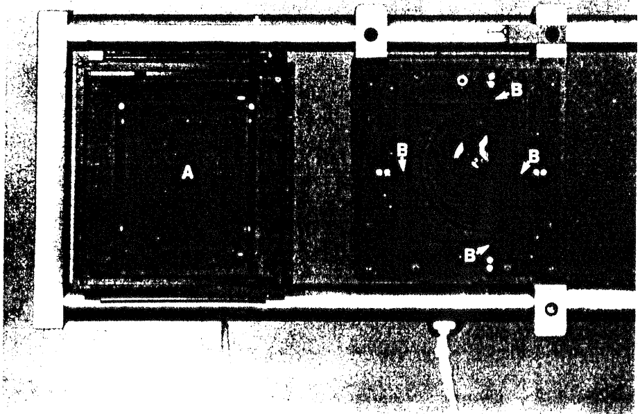
FIGURE 3. Individual camera opened to show (A) vacuum film plane, (B) fiber optic terminations for exposing the fiducial marks on the film, and (C) the scale for presetting the camera base distance
