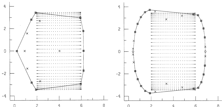
Fig. 7. Example 6.2 ( \mu = 2 , \mathbf{b} = (1, 1, \dots, 1, 1)^T ): eigenvalue estimates after 16 (left) and 32 (right) Arnoldi steps
