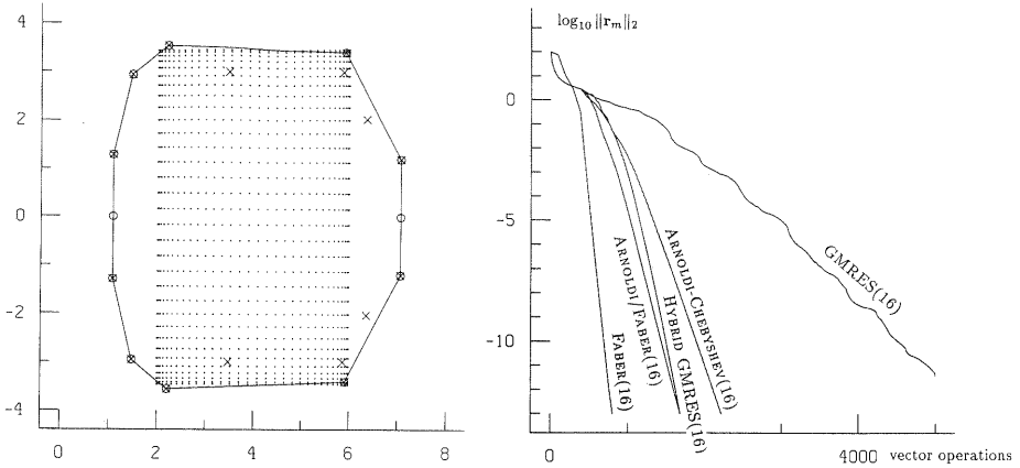
Fig. 4. Example 6.2 ( \mu = 2 ): eigenvalue estimates (left) and convergence behavior (right)
