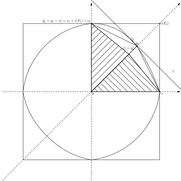
FIGURE 7. Now we have Q and Q' as in Lemma 3.6.
