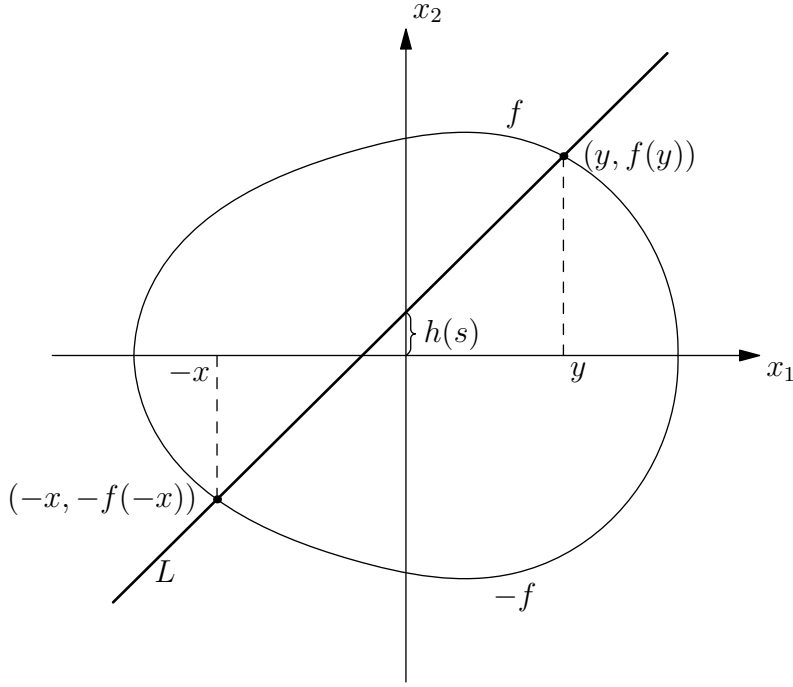
FIGURE 10. View of K and H(L) in (x_1, x_2) -plane.
