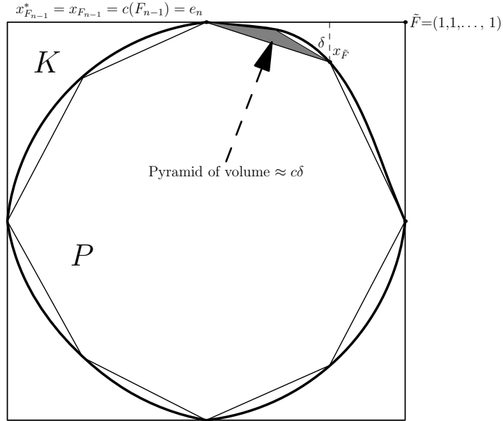
FIGURE 8. K \not\subset (1 + c\delta)P .
