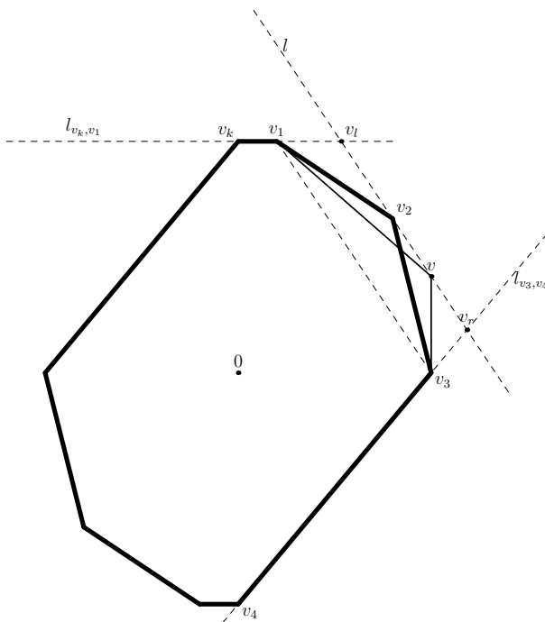
FIGURE 2. Moving vertex v_2 to vertex v along the line l , keeping |P_k(v)| constant.
