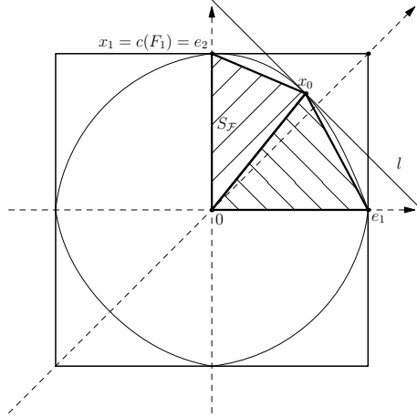
FIGURE 4. Construction of polytope P .
