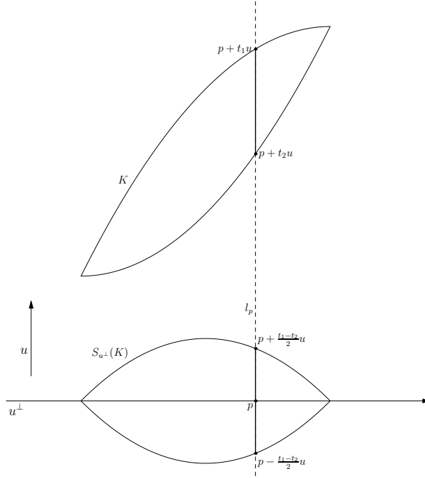
FIGURE 1. Steiner Symmetrization in \mathbb{R}^2 .
