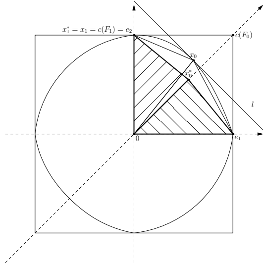
FIGURE 5. Construction of polytopes P and P' .
