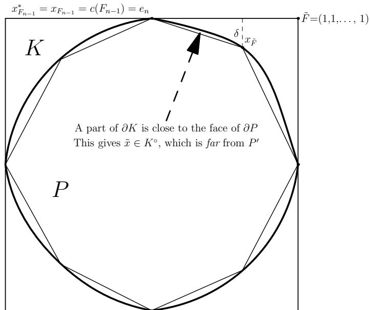
FIGURE 9. K \subset (1 + c\delta)P .
