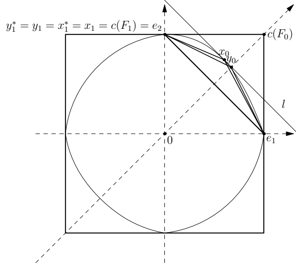
FIGURE 6. Moving x_0 to y_0 (triangle e_1, x_0, e_2 to triangle e_1, y_0, e_2 ).
