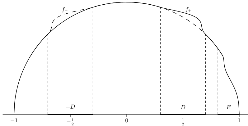
FIGURE 12. Graph of functions f_\pm
