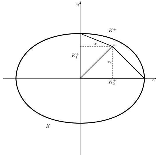
FIGURE 3. Construction of K_i^+ .
