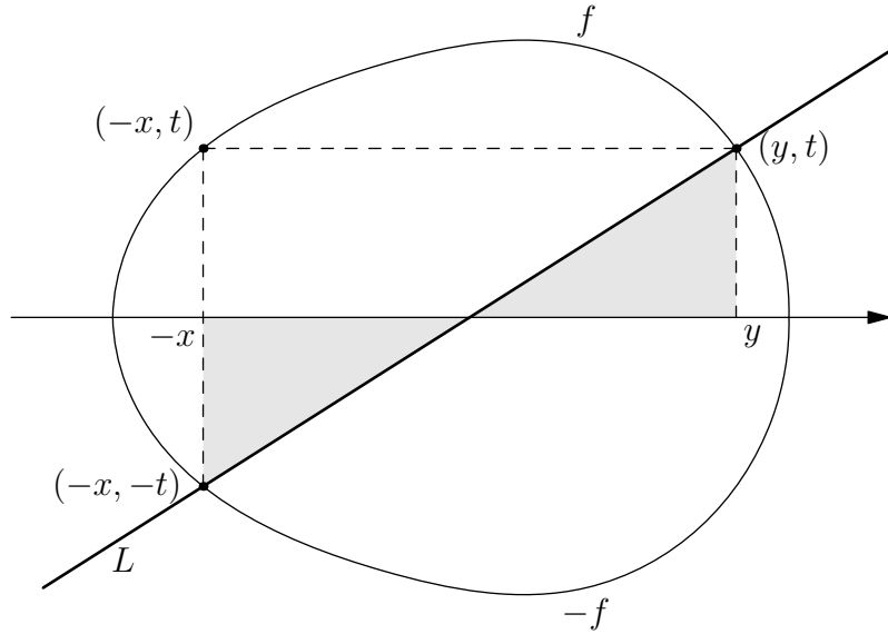
FIGURE 11. Maximal slice in \mathbb{R}^4
